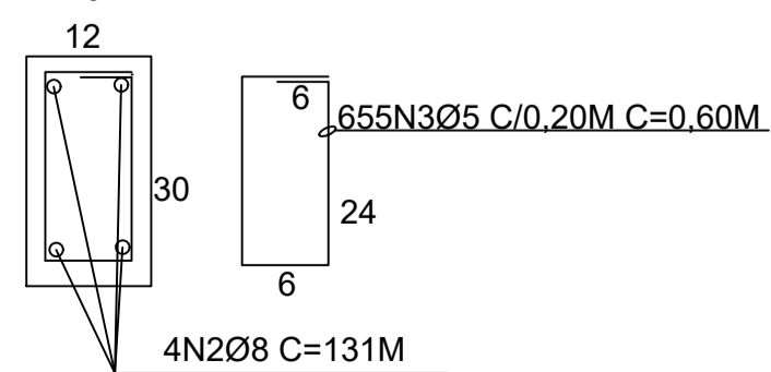
4N2Ø8 C=131M
